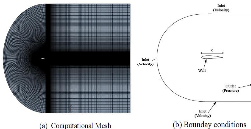
Figure 3: Computational domain meshing and boundaries.
