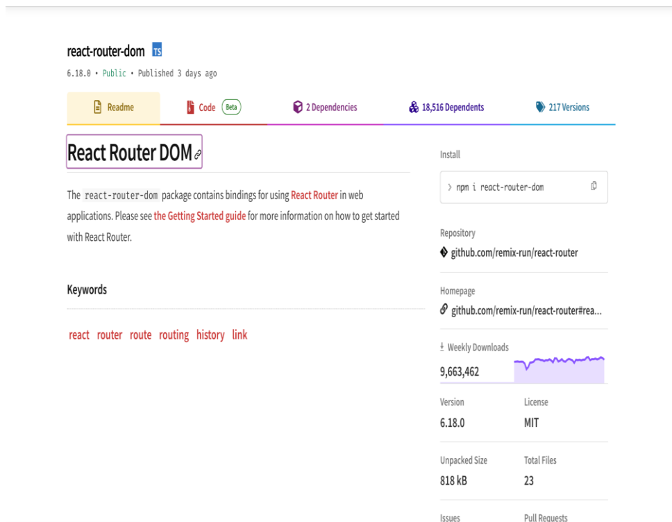
Figure 7. React-router-Dom Package
