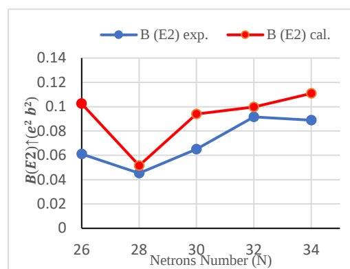
Figure 3 Comparison between B(E2)\uparrow_{\text{exp}} and B(E2)\uparrow_{\text{p. w.}} values as a function of neutrons number (N) for ^{54-62}_{28}\text{Ni} isotopes.
