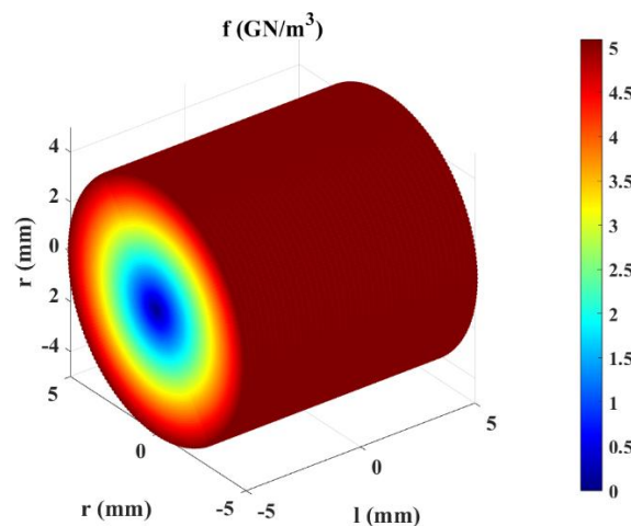
Figure 7. 3D model of Lorentz force density for a single plasma beam
