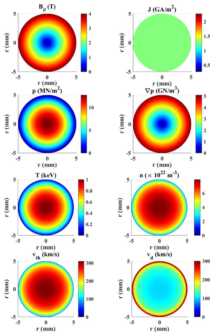
Figure 6. 2D Polar distributions of plasma parameters in a single plasma beam
