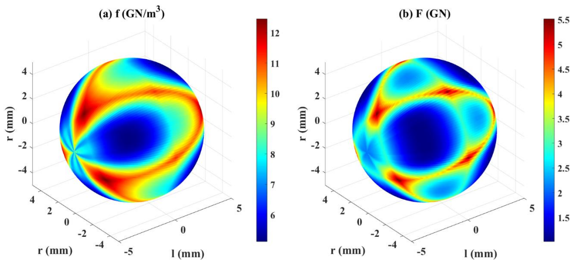
Figure 9. The in-spheres of (a) total Lorentz force density and (b) total Lorentz force acting on the focal region
