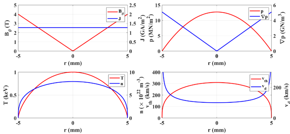
Figure 5. Radial profiles of plasma parameters in a single plasma beam
