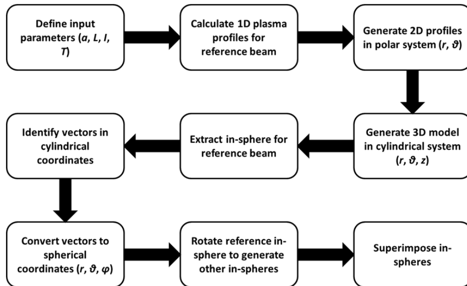
Figure 2. Graphical outline of MHD code
