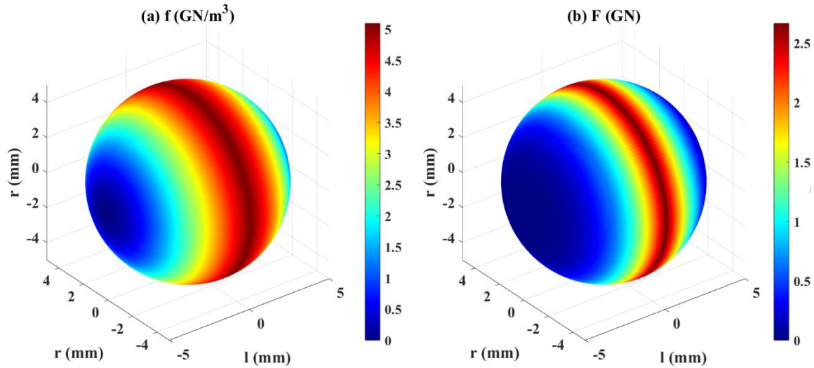
Figure 8. In-spheres of (a) Lorentz force density and (b) Lorentz force for the reference plasma beam
