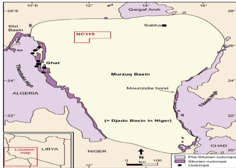
Figure 1 – Geological map of Murzuq Basin showing the location of NC115 Concession [4].
