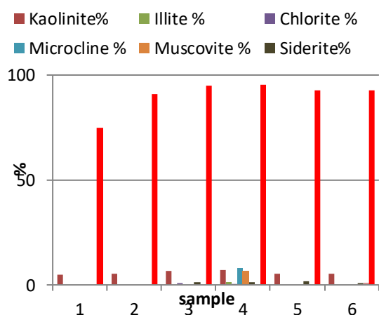
Figure 8. Bar graph representation the relative percentages of the bulk minerals in the Mamuniyat Formation.
