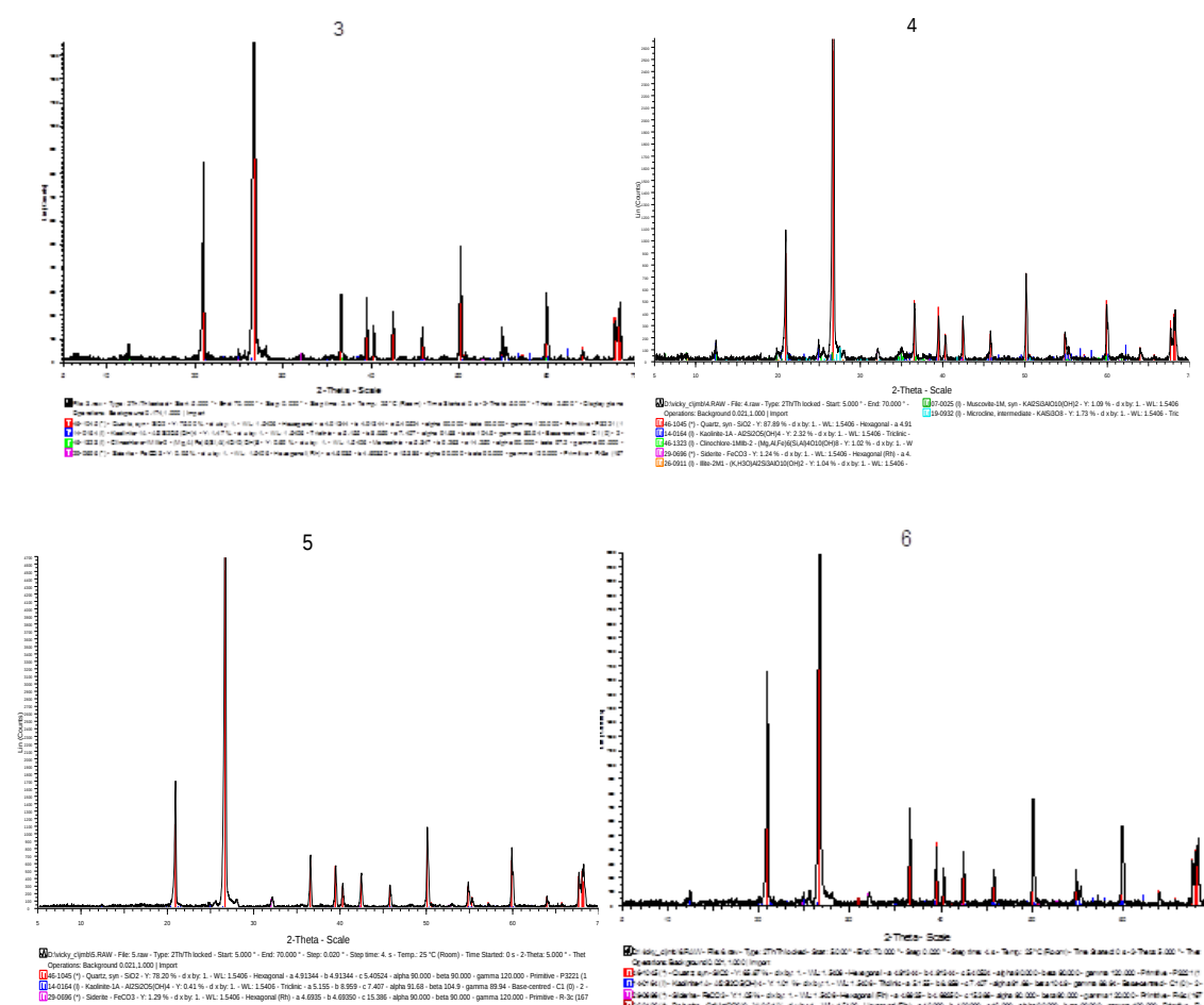
Figure 2. X-ray diffractogram of clay samples 3,4,5,6 (well B1)
