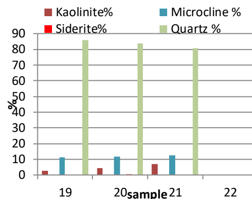
Figure 11. Bar graph representation the relative percentages of the bulk minerals in the Mamuniyat Formation.
