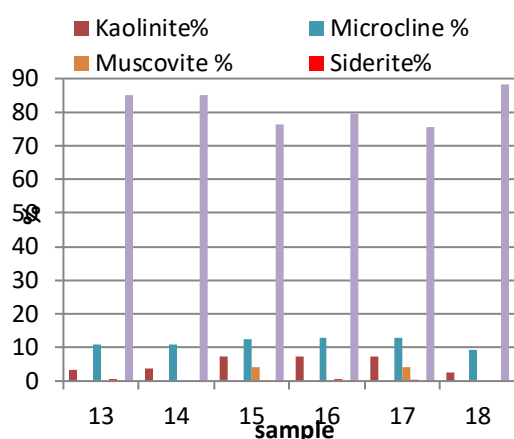
Figure 10. Bar graph representation the relative percentages of the bulk minerals in the Mamuniyat Formation.
